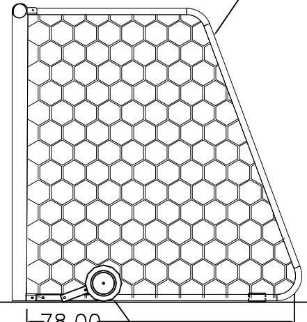
10" TRANSPORT WHEEL
