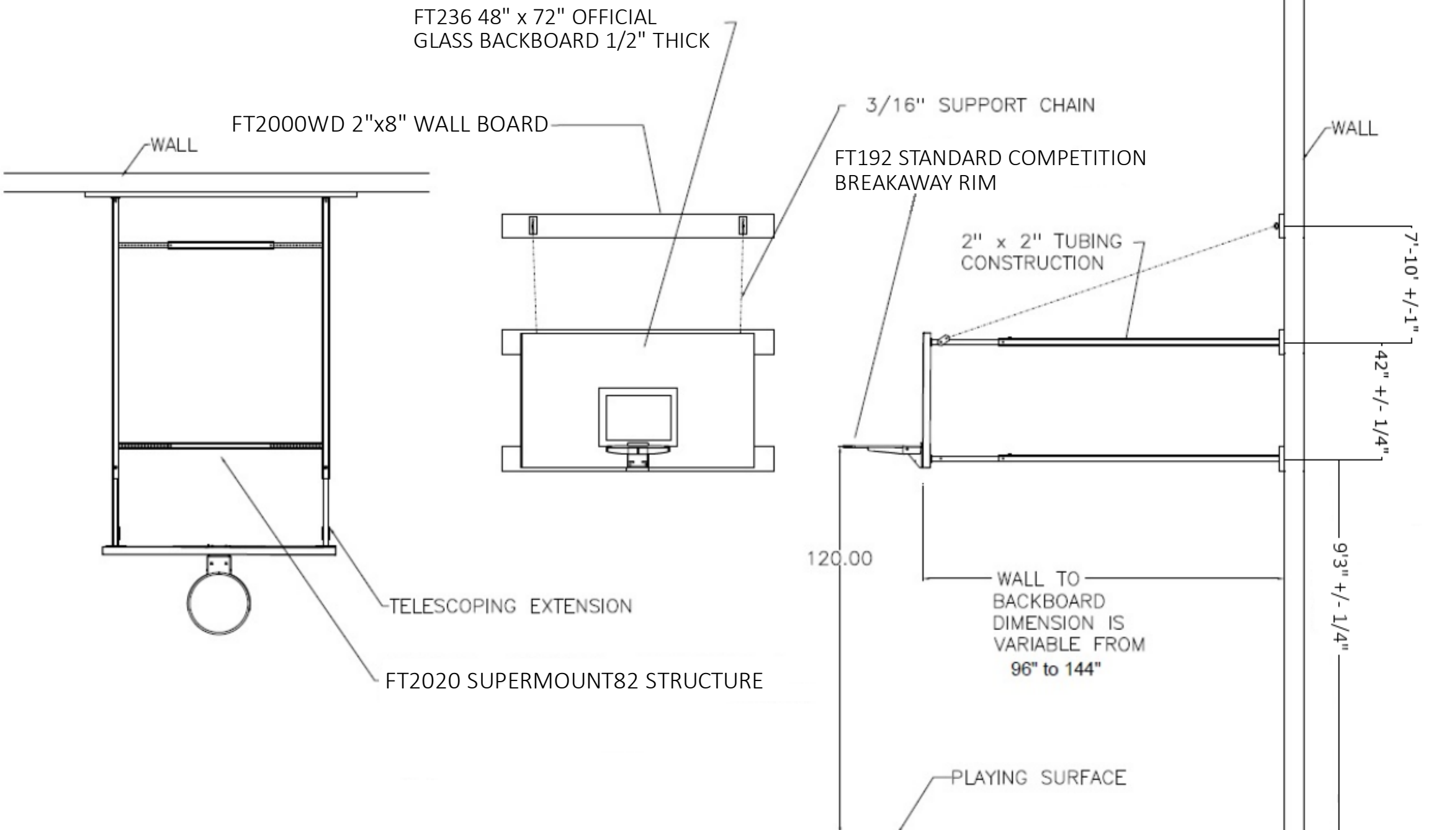
FRONT VIEW
