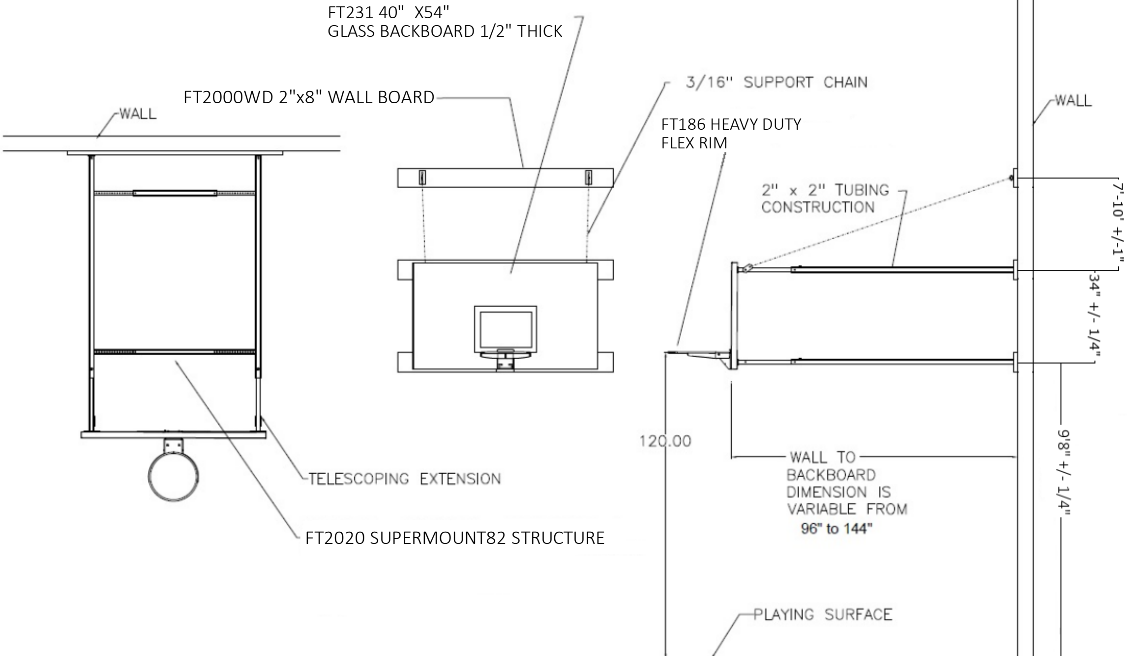
FRONT VIEW
