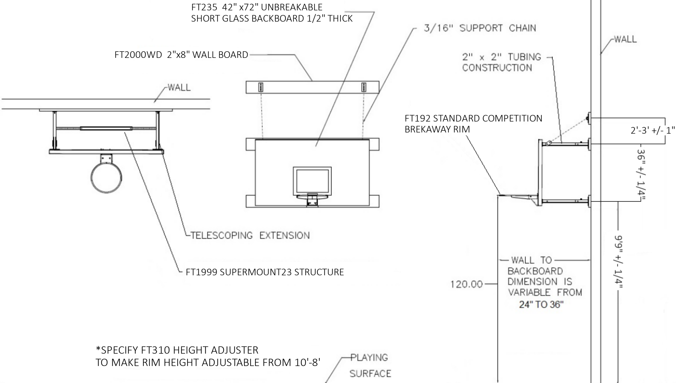
FRONT VIEW
